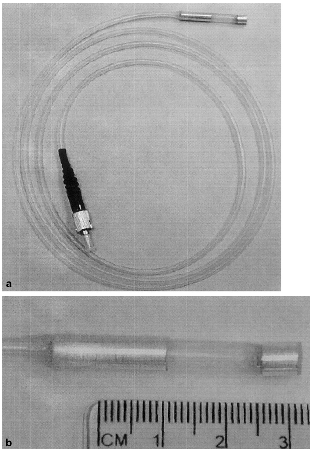
Figure 2. a: The fiber-optic cardiac pacing lead. b: Close-up showing the tip and ring electrodes for the fiber-optic cardiac pacing lead (Reproduced with permission from Greatbatch et al., JMRI 2002;16:97-103).
